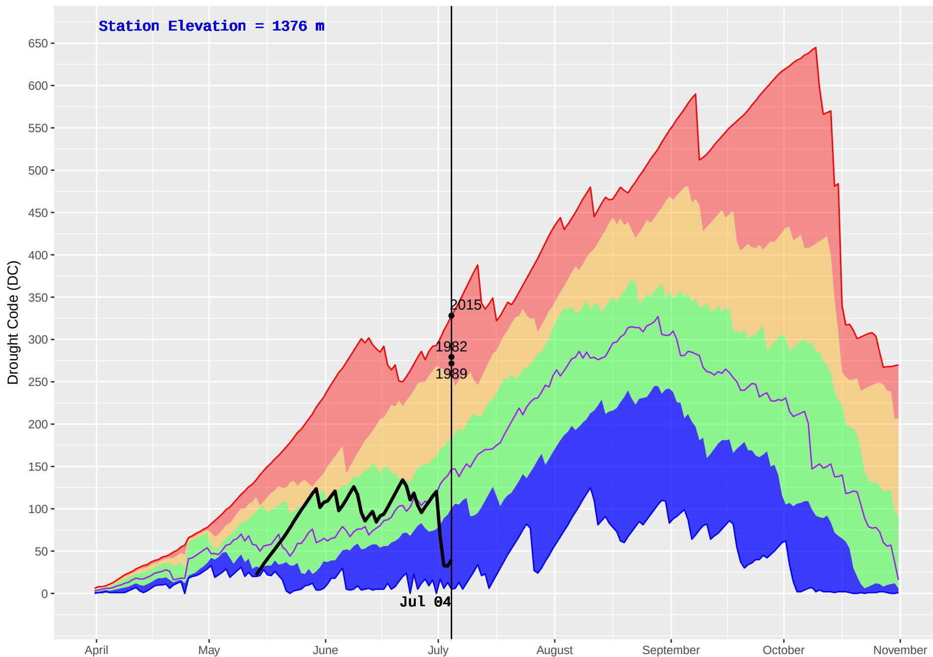
DUNCAN (385) : Historical (1981–2016) and Current (2018) Noon Drought Code (DC)
